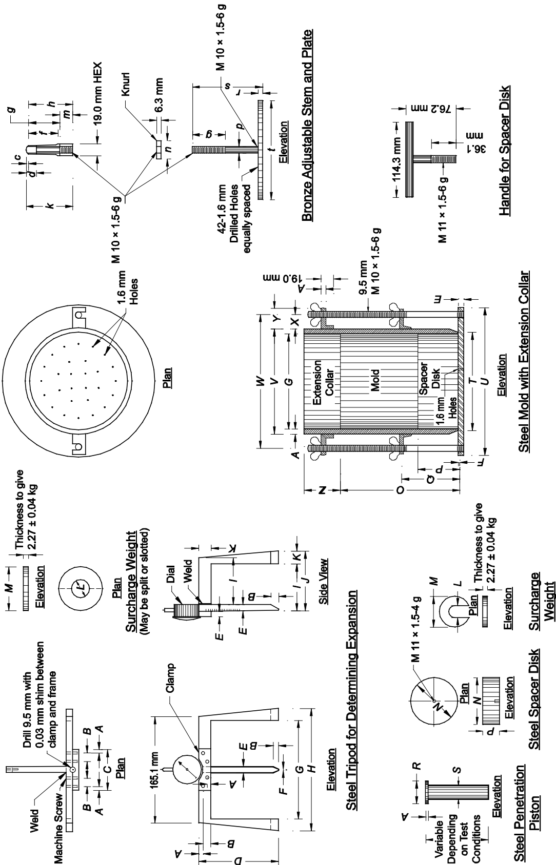
Figure 1—California Bearing Ratio Apparatus
