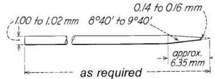
FIG. 1 Needle for Penetration Test
